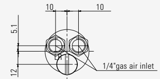
Air exhaust silencer
