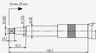
3/8" square drive axial compensator (Din 3121-F 10) (cod.680601070)
